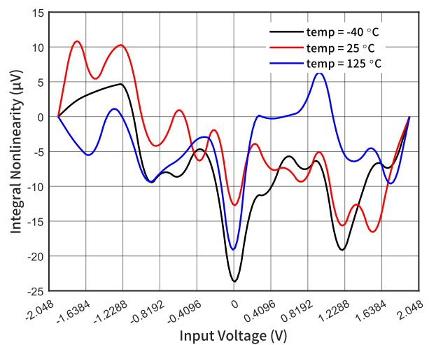
图 7 INL vs 输入电压 (VDD = 3.3, FSR = ±2.048V)
